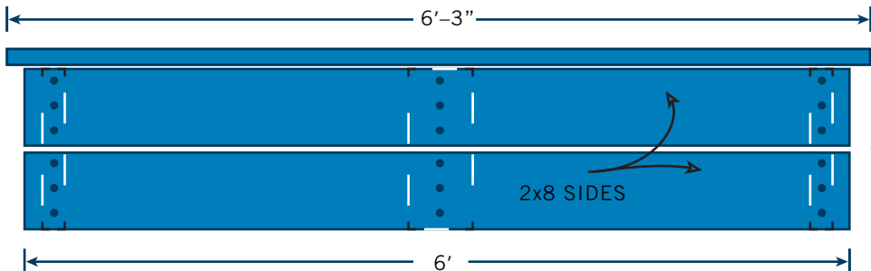
FRONT VIEW
